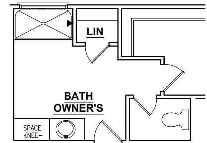
Optional Owners Bath with 5' Shower
