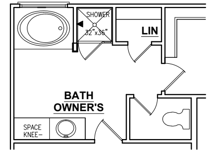
Optional Owners Bath with Separate Tub/ 36" Shower
