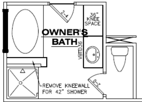
Optional Owner's Bath with " Garden Tub & 36" Shower
