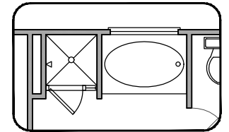
OPTIONAL DELUXE OWNER'S BATH W/ GARDEN TUB & 36" SHOWER
