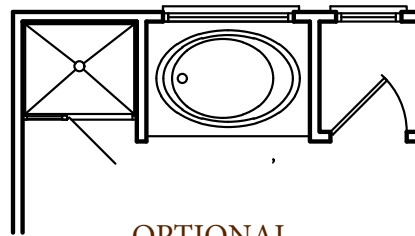
OPTIONAL OWNER BATH GARDEN TUB & SEPERATE 36" SHOWER
