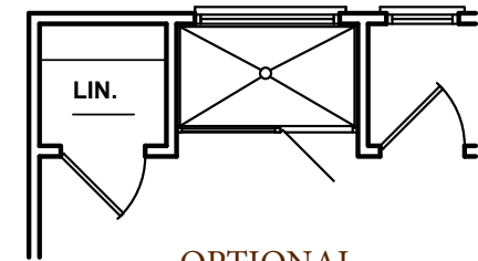
OPTIONAL OWNER BATH W/6036 SHOWER & LINEN CLOSET
